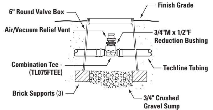
Air/Vacuum Relief Vent - 1/2" MPT TLAVRV
